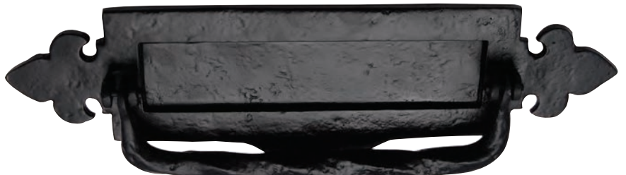
TC772 Letter Plate Fleur de Lys with Knocker 371 x 112mm - CtoC 285mm Aperture 208 x 48mm
