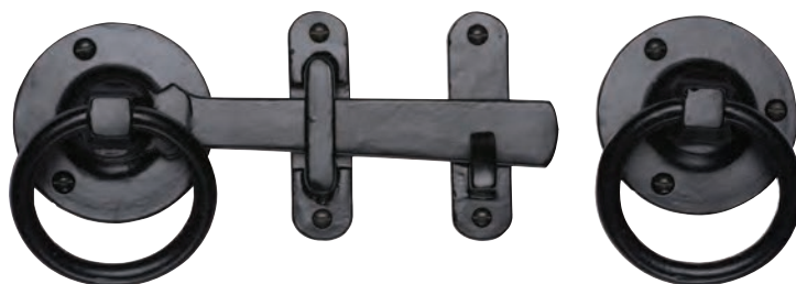
FB541 Ring Handle and latch Handle diameter: 72mm Latch length: 170mm
