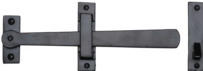
FB571 Gate handle and latch Handle: 218 x 50mm Latch length: 218mm
